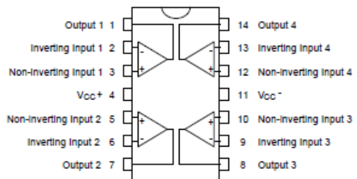
Pin connections (Top view)
