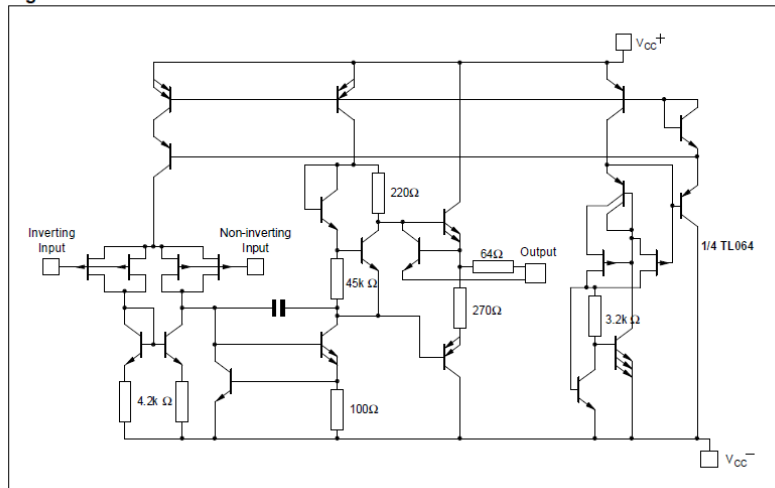
Figure 1. Circuit schematics
